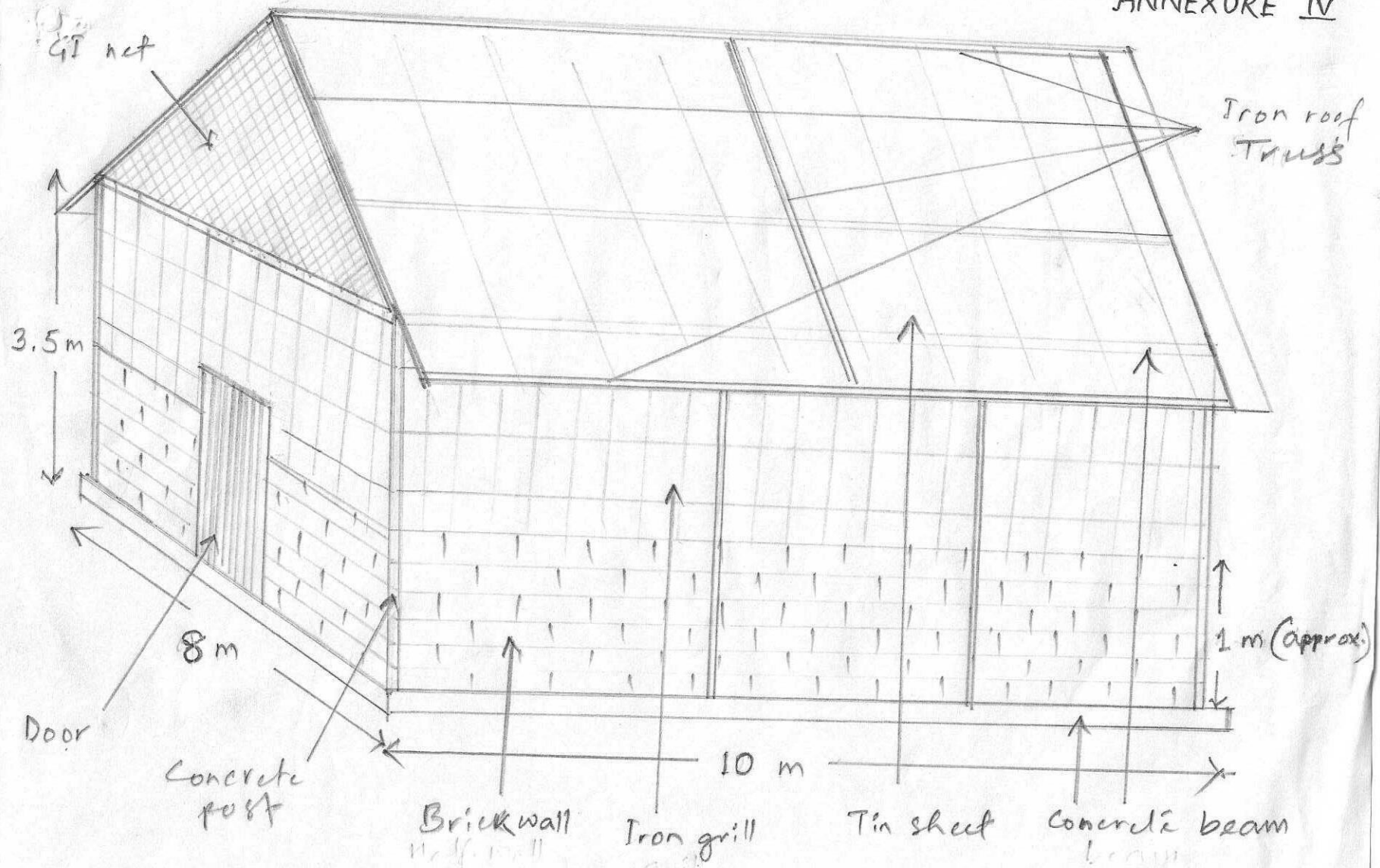
Fig: Layout of Shed house - Biofloc Unit (including 4 tanks inside)
